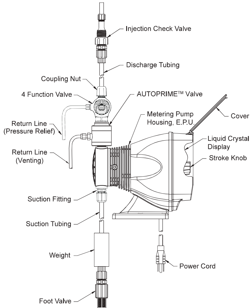
Metering Pump Component Diagram
