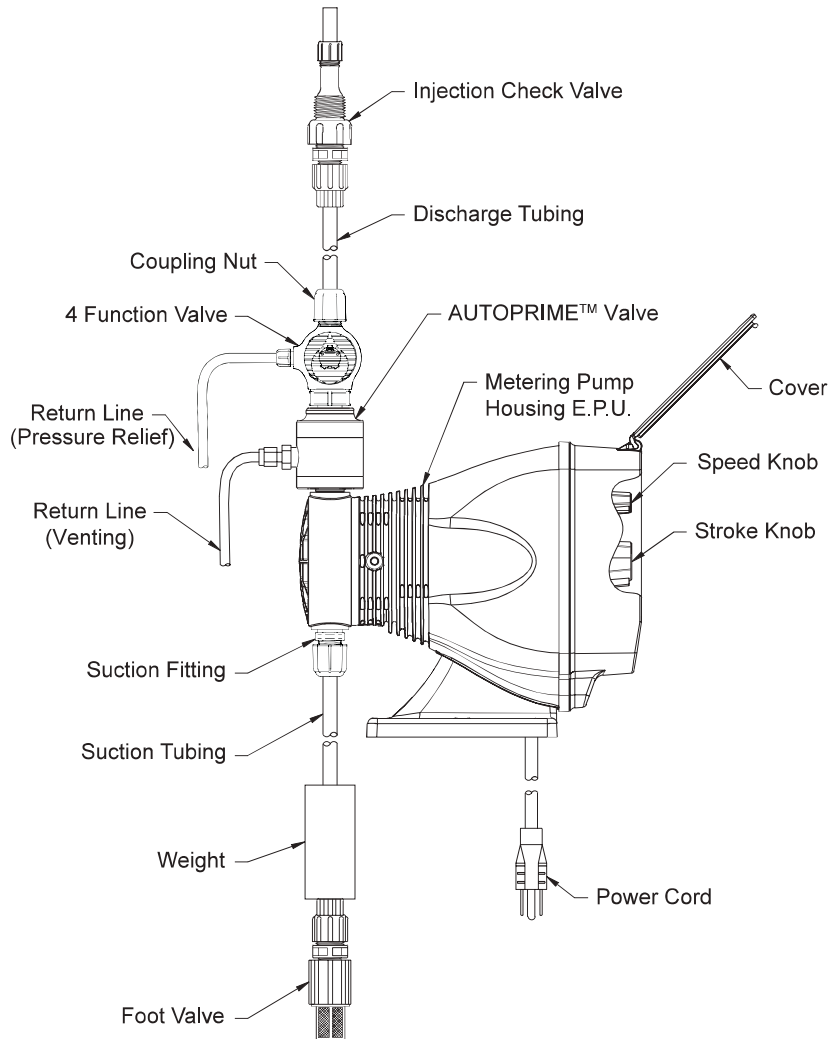
Metering Pump Component Diagram
