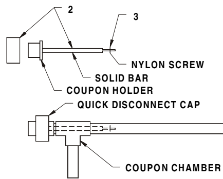
COUPON DETAIL
